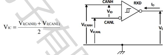
Receiver Voltage and Current Definitions
