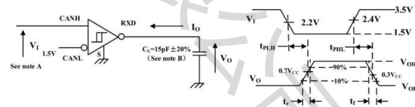
Receiver test circuit and voltage wave
