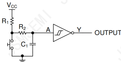
Figure 2. Push Button Debounce Circuit Schematic
