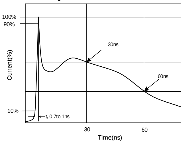
Figure2: ESD pulse waveform according to IEC 61000-4-2
