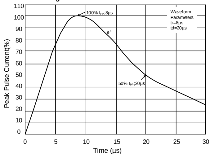
Figure1: 8/20μs pulse waveform according to IEC61000-4-5
