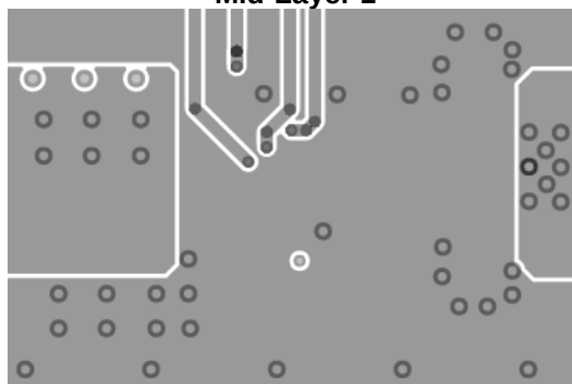
Mid-Layer 2
