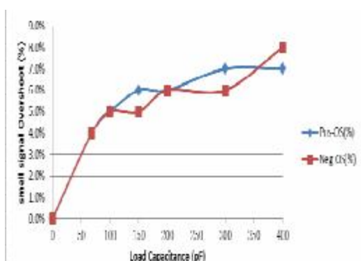
Overshoot (OS) vs Load Capacitance
