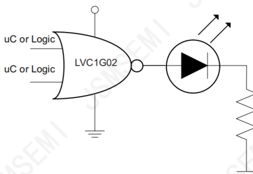
Basic LED Driver
