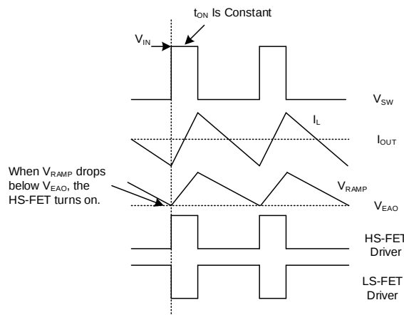
Figure 3: PWM Operation
