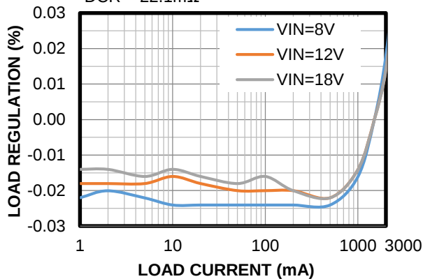
Load Regulation
