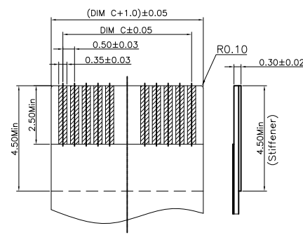
RECOMMENDED FFC/FPC
