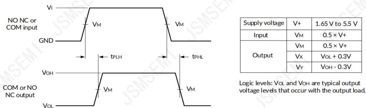
Figure 6. Propagation delay (t pd )
