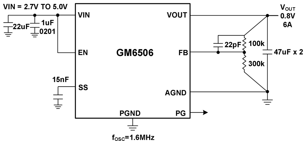
图 17. V IN =3.3V, V OUT =0.8V, I LOAD =6A
