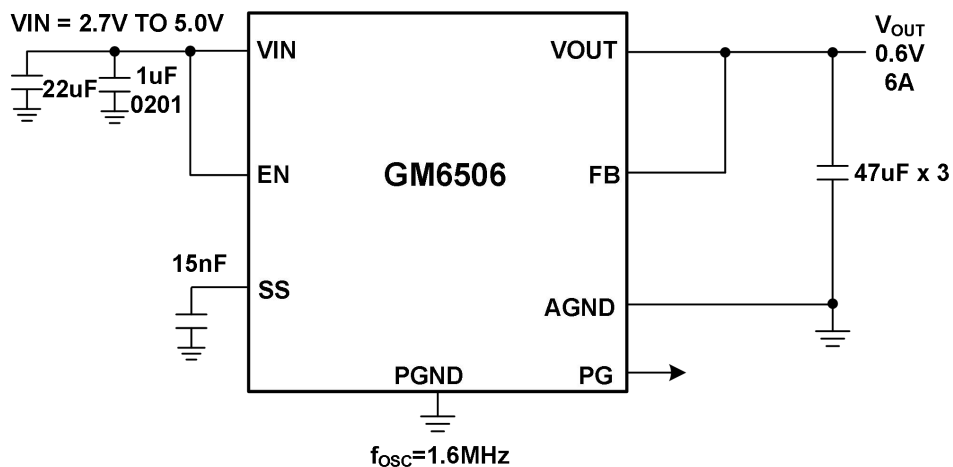
图 18. V IN =3.3V, V OUT =0.6V, I LOAD =6A
