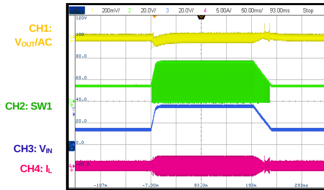
Input Voltage Transient
