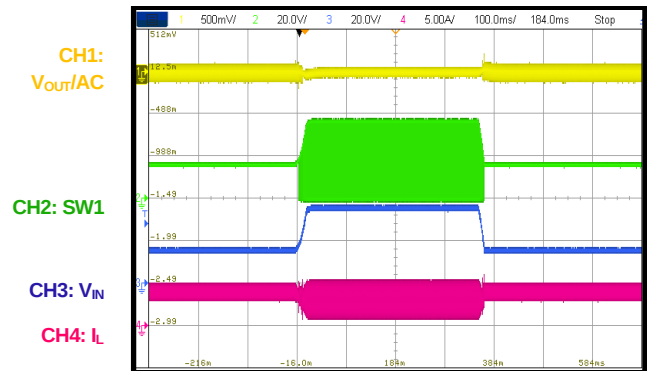
Input Voltage Transient
