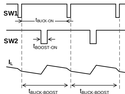
Figure 4: Buck-Boost Waveform
