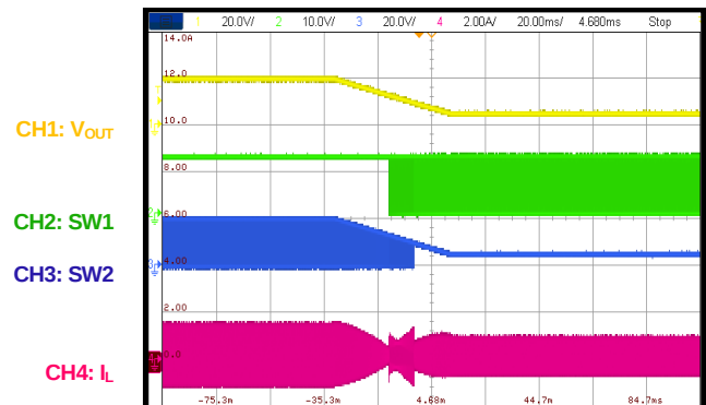
Output Voltage Transition
