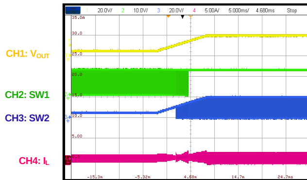
Output Voltage Transition
