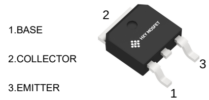
TO-252-2L (DPAK)
