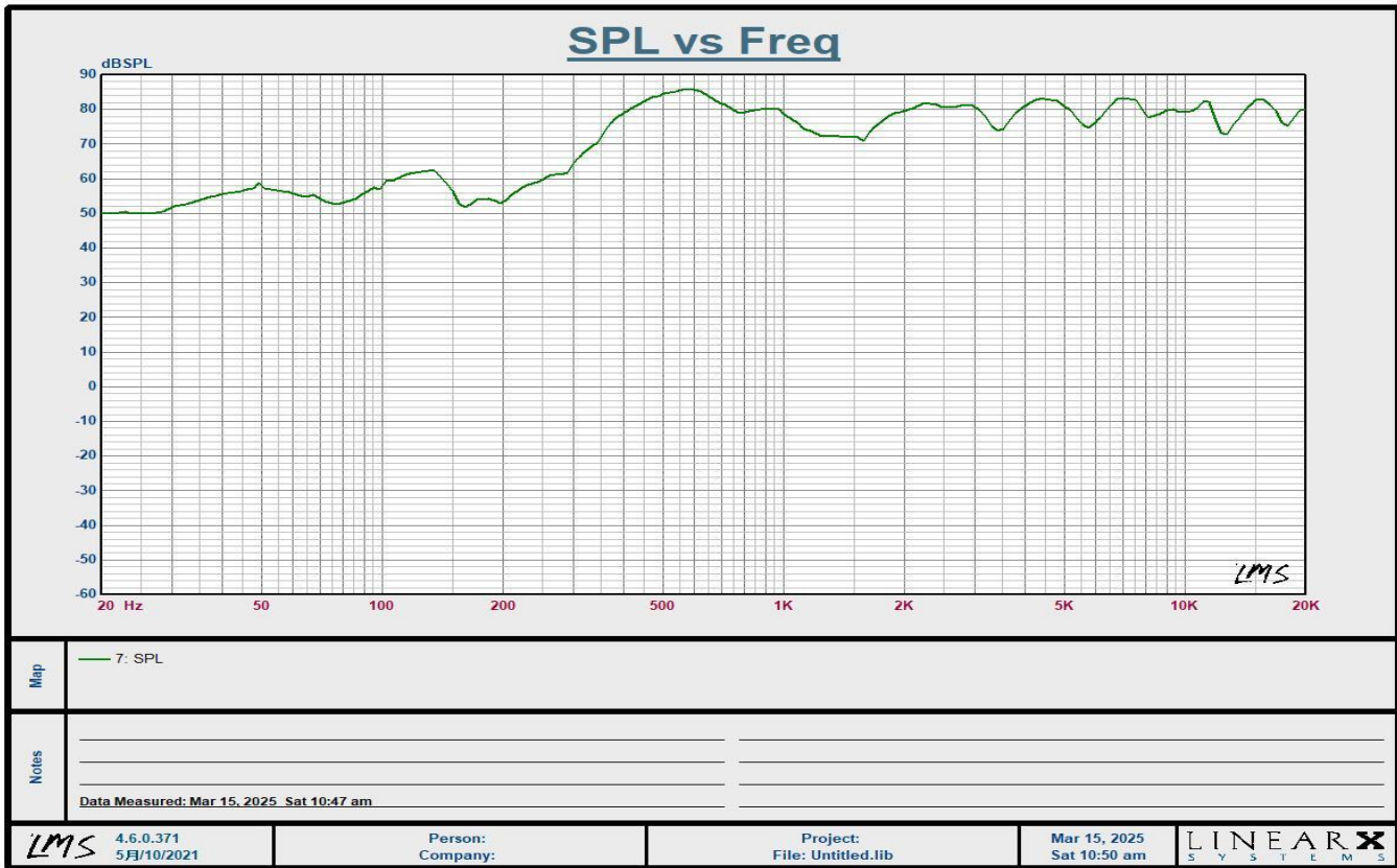
频响曲线图 Frequency response curve
