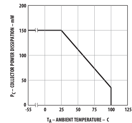
Figure 2: Collector Power Dissipation vs. Temperature
