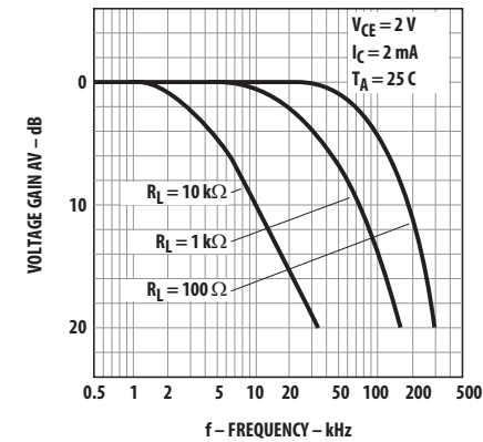
Figure 11: Frequency Response
