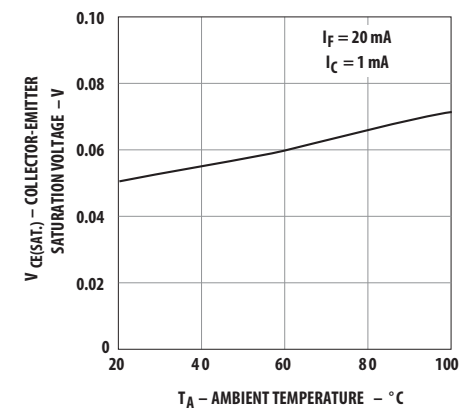
Figure 8: Collector-Emitter Saturation Voltage vs. Temperature
