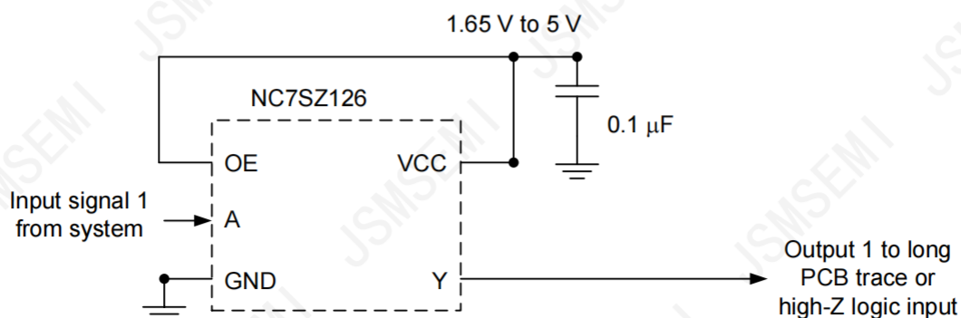
Figure 2. Application Schematic
