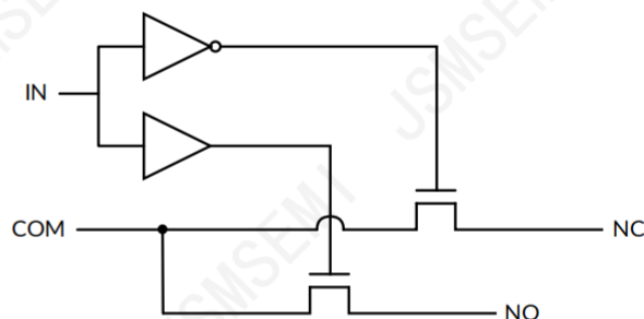
Simplified Schematic
