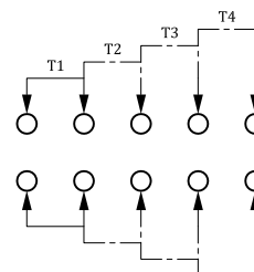
SCHEMATIC(SHORTING)
