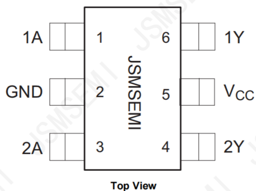
Pin Functions
