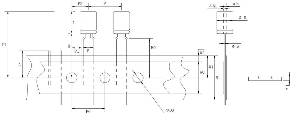
[ Fig. 1 (Diameter for Φ4 to Φ8)]
