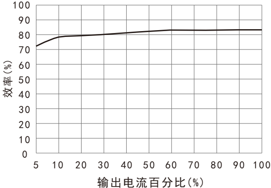
效率Vs输出负载(V in =5V) VRA0512YMD-10WR3
