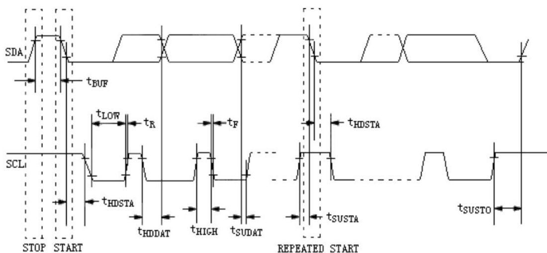
Timing diagram figure 8
