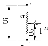
Figure 2A used for vottage divider(recommended)
