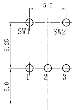
P. C. B. MOUNTING DETAIL
