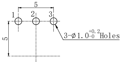
P.C.B MOUNTING DETAIL
