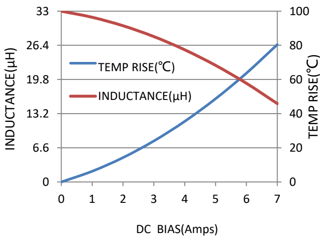
MAWH-1050-330-M-5A
