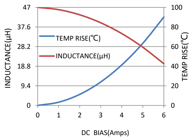
MAWH-1050-470-M-5A
