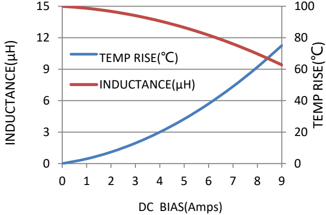
MAWH-1050-150-M-5A
