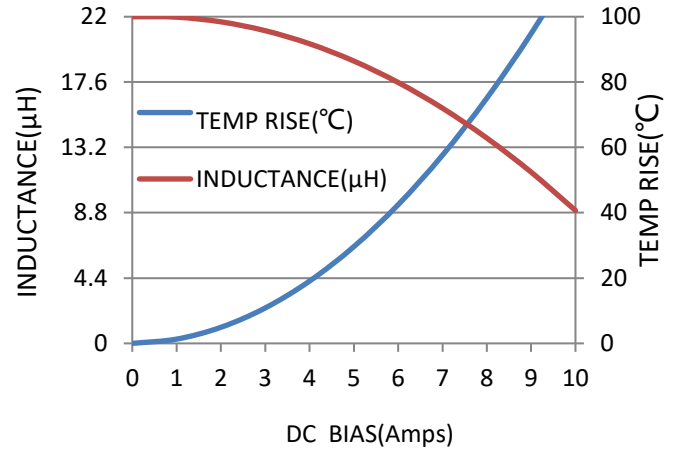
MAWH-1050-220-M-5A
