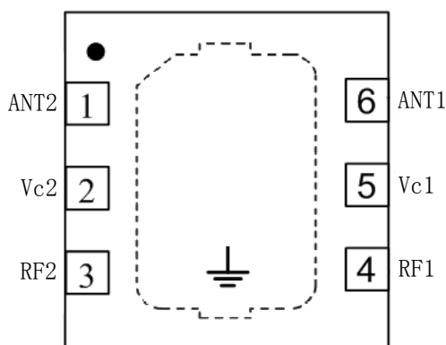
Figure 1. GSR1411S Pin-Def. (Top View)
