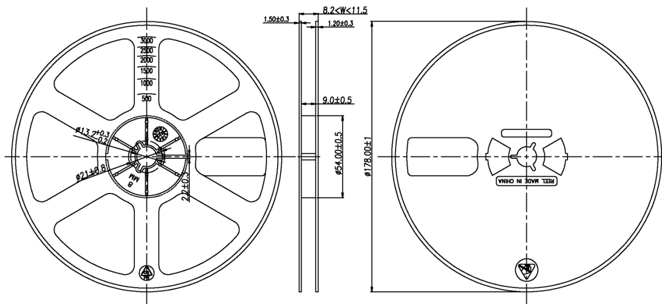
Figure 5. GSR1411S Tape and Reel Dimensions
