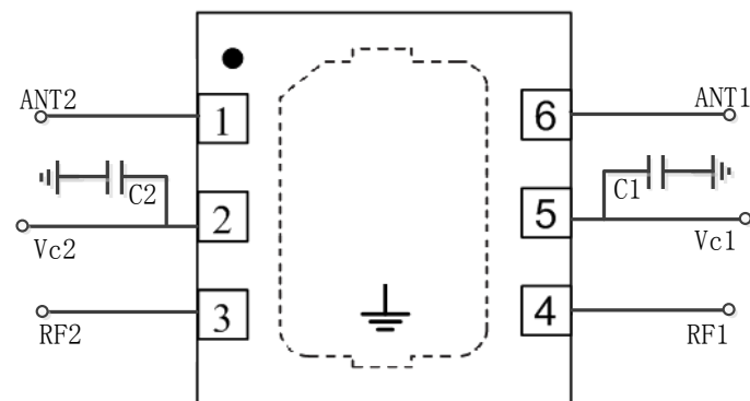
Figure 2. GSR1411S Pin Out
