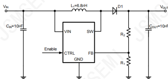
Typical Boost Application Circuit
