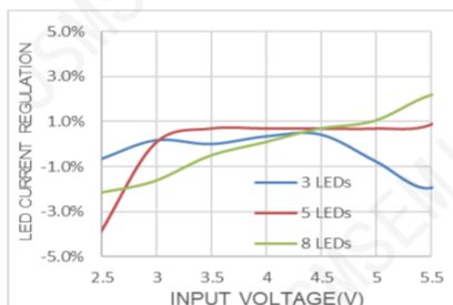
LED Current Regulation vs. Input Voltage
