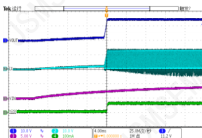
V_{IN} Startup
