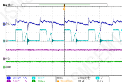
Steady State Operation
