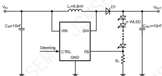
Typical White LED Application Circuit
