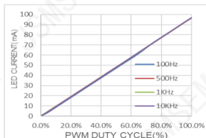
LED Current vs. PWM Duty Cycle
