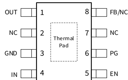
Figure 3 NSR332 Series Pin-out
