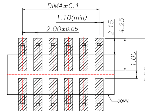
SUGGESTED PCB LAYOUT (COMPONENT SIDE) 适用线路板(厚度:1.6mm)
