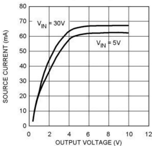
Source Current vs. Output Voltage
