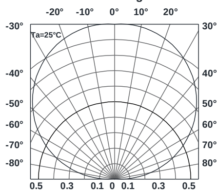
Radiation Diagram
