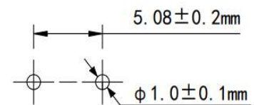
PCB板上的孔 HOLES IN THE PCB BOARD
