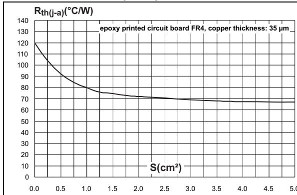
Figure 6. Thermal resistance junction to ambient versus copper surface under each lead (SMA)
