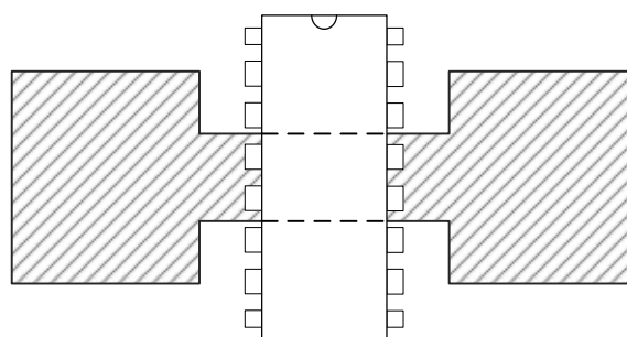
Layout Example of PCB Copper Area (Used as Heat Sink)
