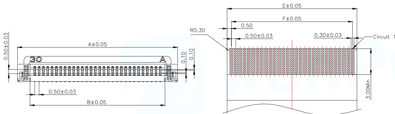
RECOMMENDED FPC/FFC DIMENSION
