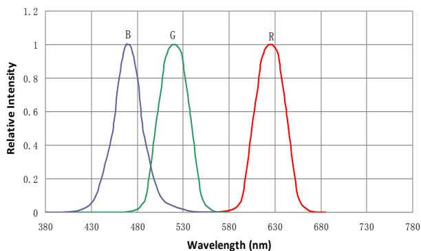
Spectrum Distribution ( T_a=25^{\circ}\text{C} )
