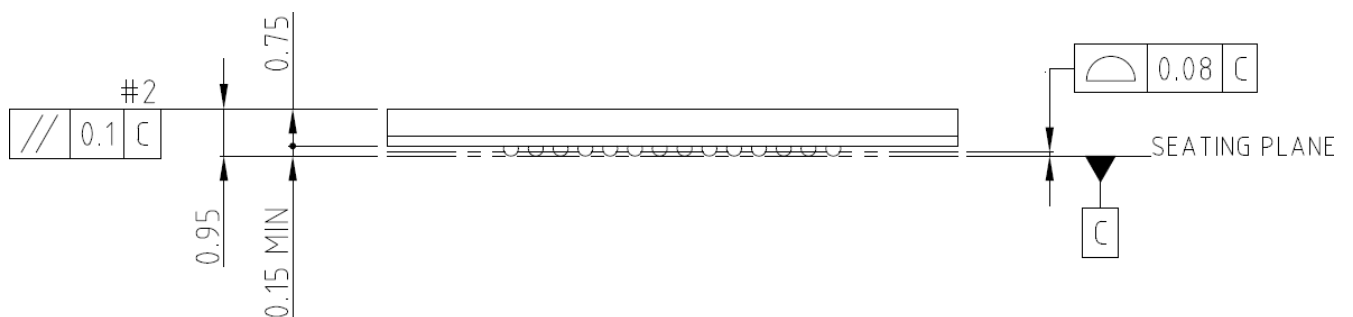
Figure 5 11.5 x 13.0 x 1.0mm Bottom & side View
