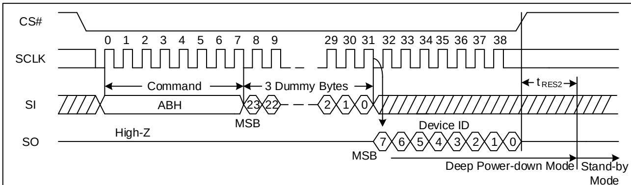
Figure 34. Release Power-Down/Read Device ID Sequence Diagram
