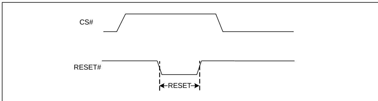
Figure 2 RESET Condition
