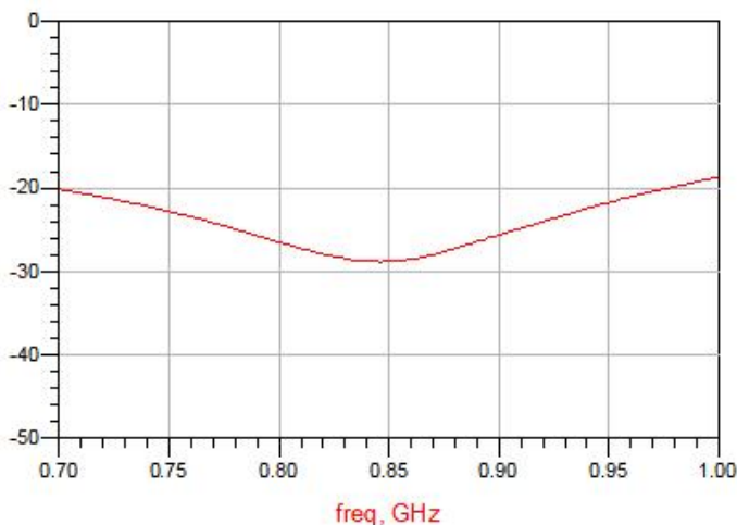
Figure 5. MPD0710W2 Return Loss (S2, 2)
