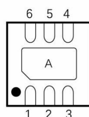
Figure 1. MPD0710W2 Port Configurations (Top View)
