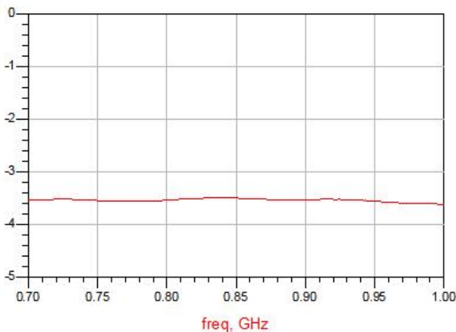
Figure 3. MPD0710W2 Insertion Loss (6, 2)
