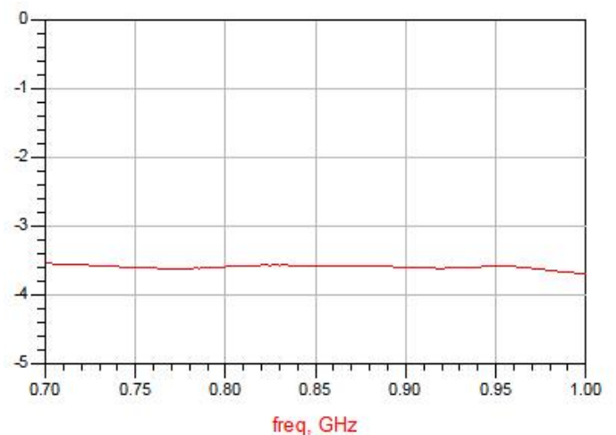
Figure 4. MPD0710W2 Insertion Loss (4, 2)
