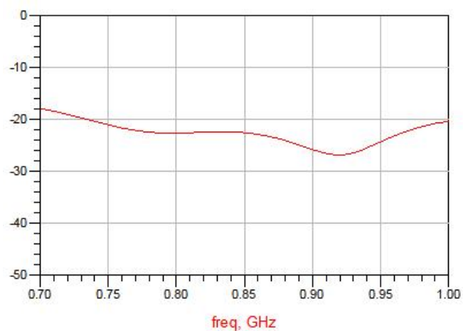
Figure 8. MPD0710W2 Isolation (S4, 6)
