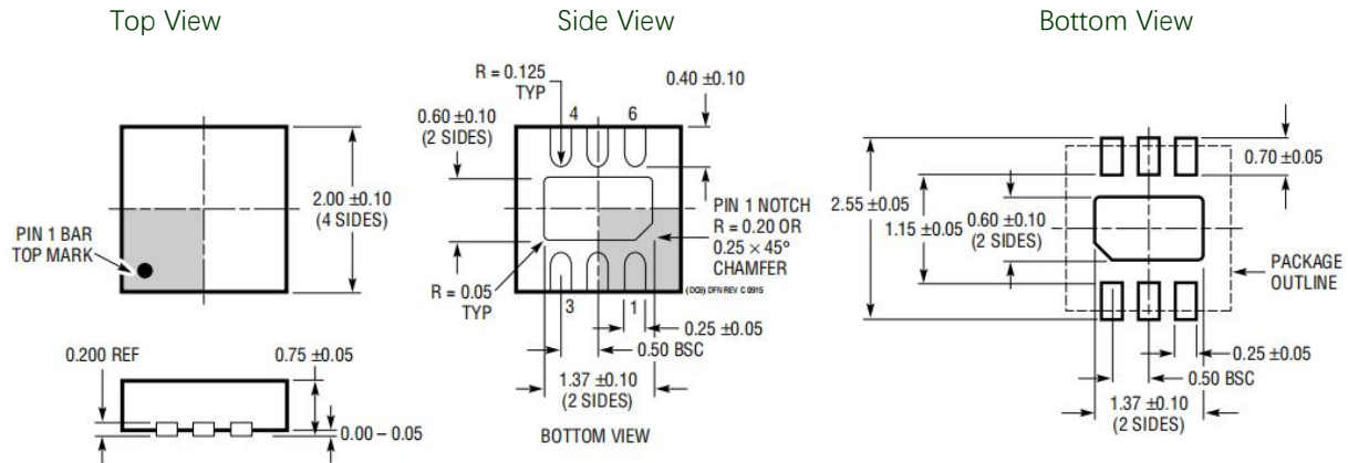
Figure 2. MPD0710W2 Outline Drawing
