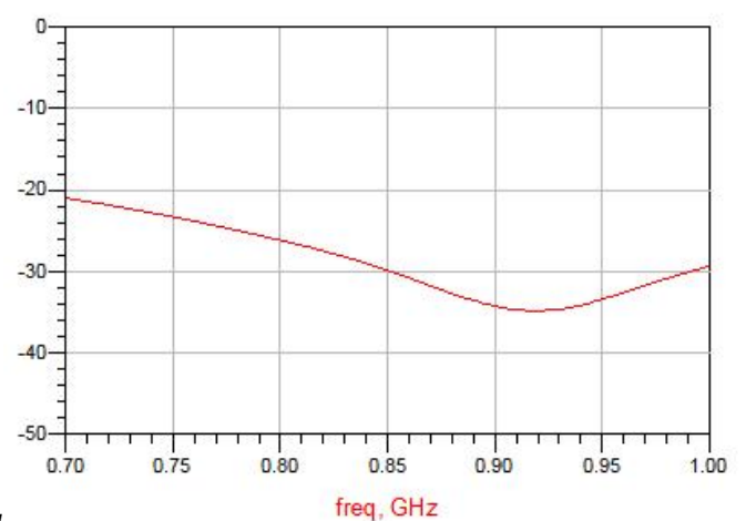
Figure 6. MPD0710W2 Return Loss (S4, 4)
