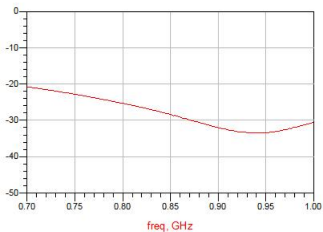
Figure 7. MPD0710W2 Return Loss (S6, 6)
