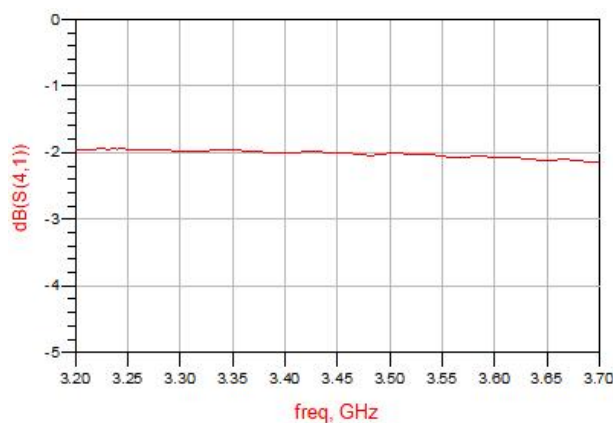
Figure 3. MHC35X02 Coupling
