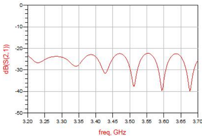
Figure 9. MHC35X02 Isolation
