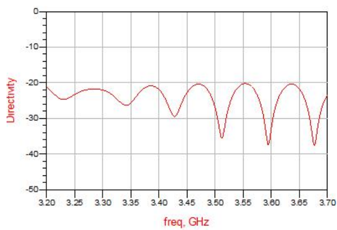
Figure 12. MHC35X02 Directivity
