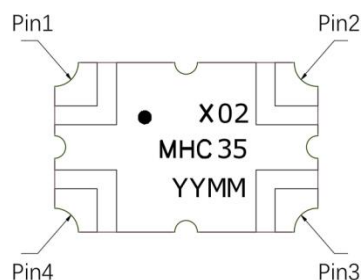
Figure 1. MHC35X02 (Top View)
