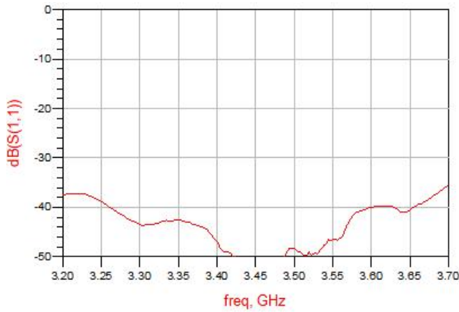
Figure 5. MHC35X02 Return Loss (S11)
