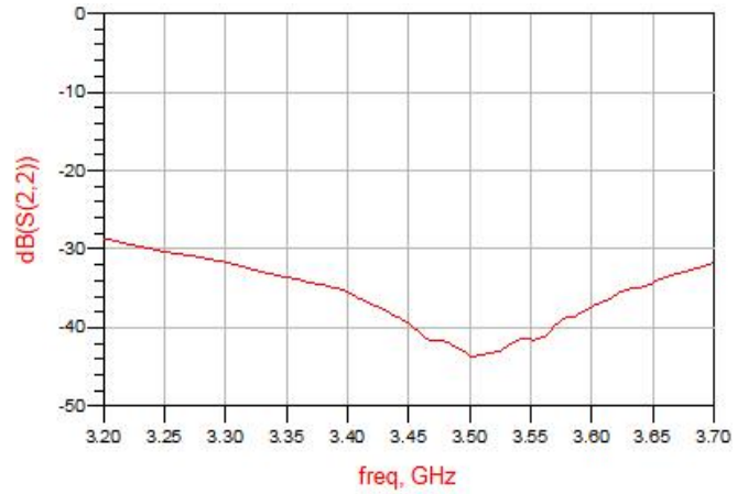
Figure 6. MHC35X02 Return Loss (S22)
