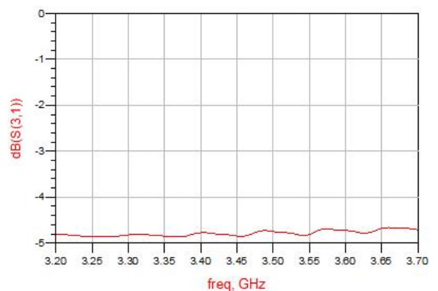
Figure 4. MHC35X02 Transmission
