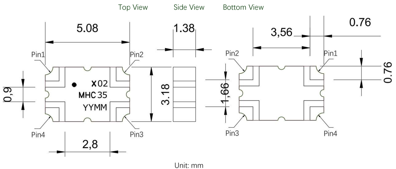
Figure 2. MHC35X02 Outline Drawing
