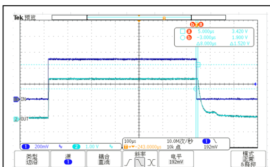
Positive Overload Recovery
