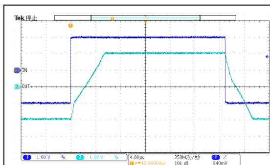
Large Signal Response
