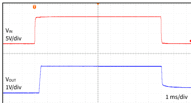
Figure 14 Line Transient
