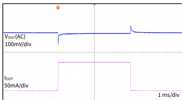
Figure 15 Load Transient
