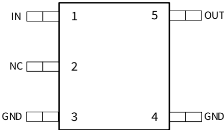
Figure 2 SOT-23-5L (NSR310 Version) Pin-out (Top View)
