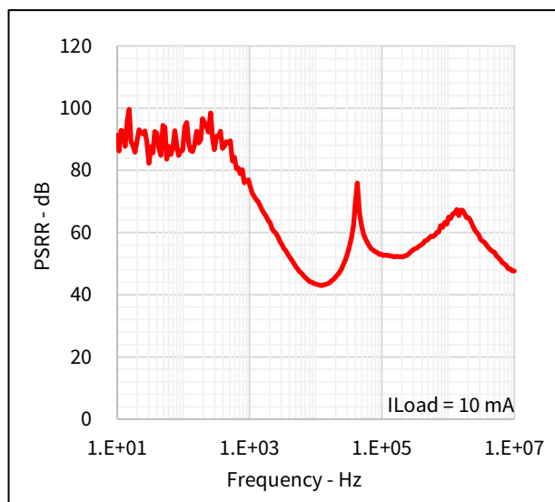
Figure 13 Power Supply Rejection Ratio (PSRR)
