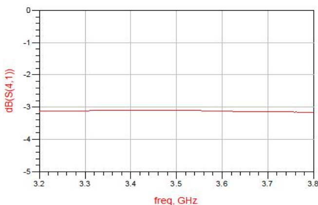
Figure 3. MHC35X03 Coupling
