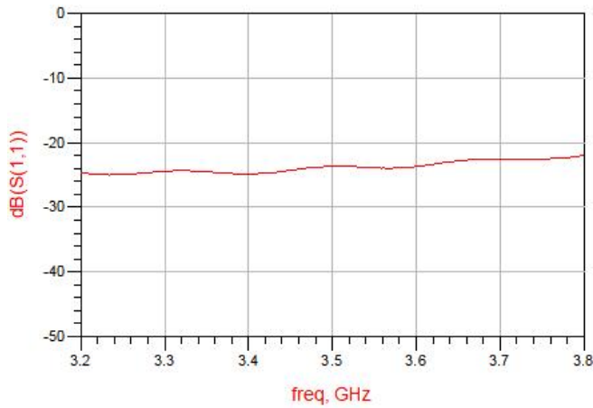
Figure 5. MHC35X03 Return Loss (S11)
