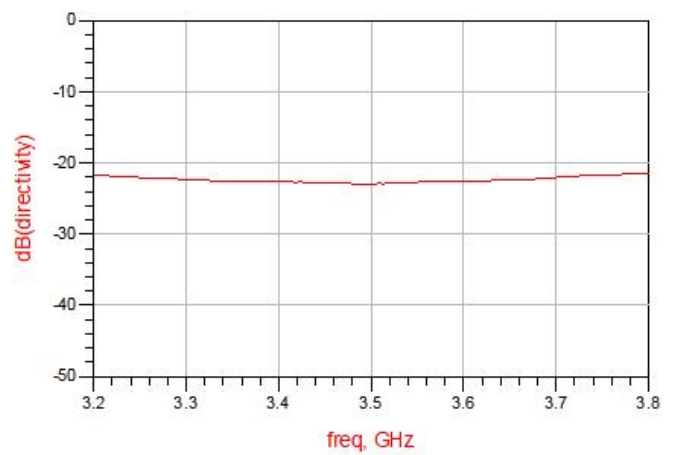
Figure 12. MHC35X03 Directivity
