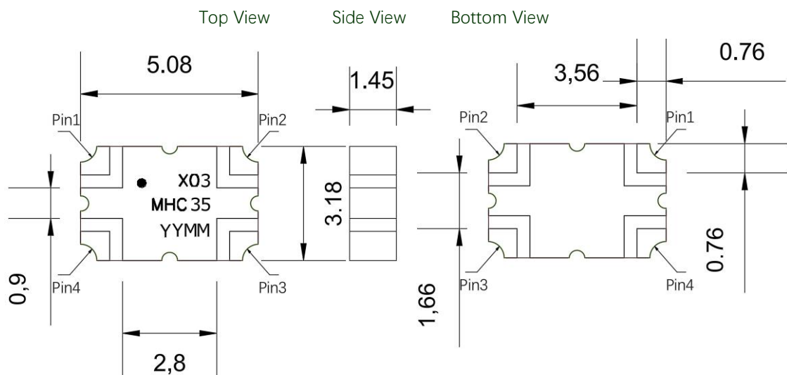
Figure 2. MHC35X03 Outline Drawing
