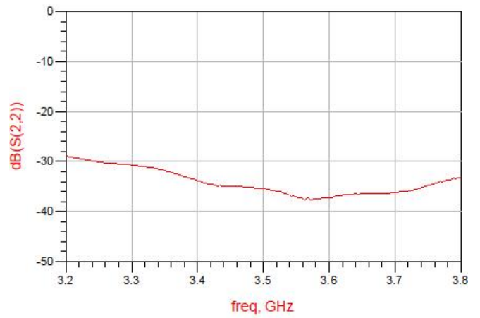
Figure 6. MHC35X03 Return Loss (S22)
