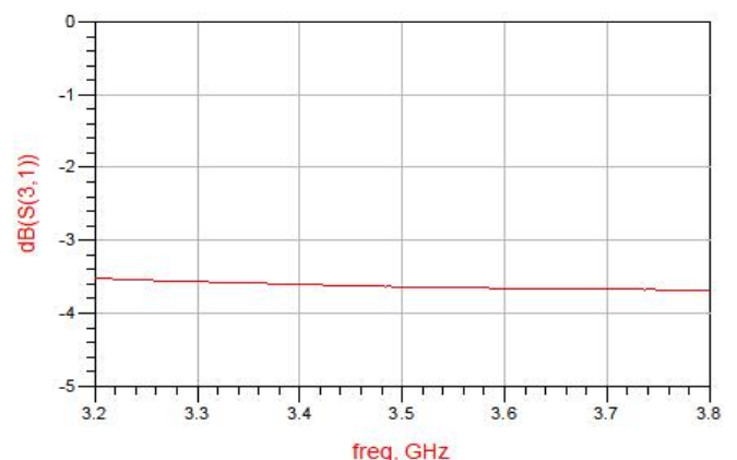
Figure 4. MHC35X03 Transmission
