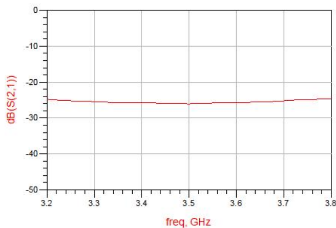
Figure 9. MHC35X03 Isolation
