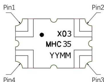
Figure 1. MHC35X03 (Top View)
