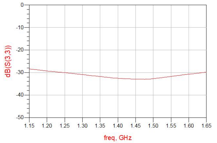
Figure 6. MHC14S03 Return Loss (S33)
