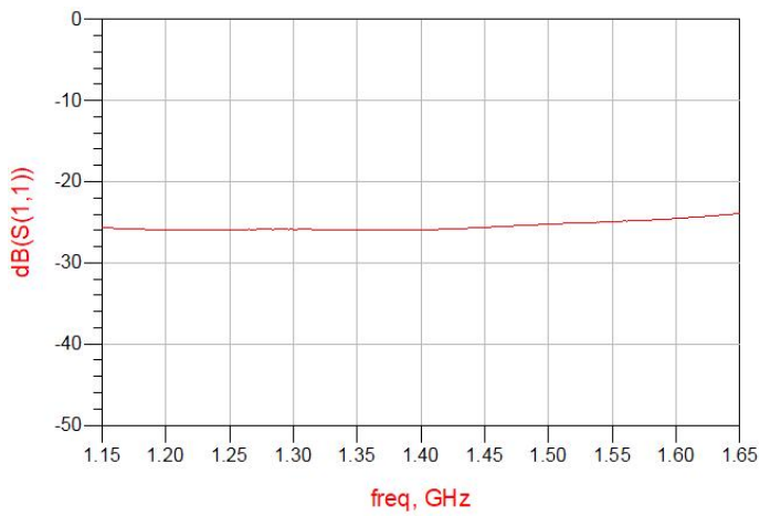
Figure 5. MHC14S03 Return Loss (S11)
