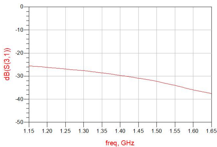
Figure 9. MHC14S03 Isolation
