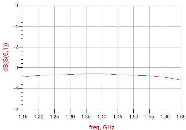
Figure 3. MHC14S03 Coupling
