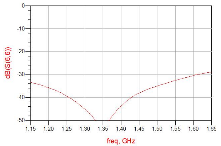
Figure 8. MHC14S03 Return Loss (S66)
