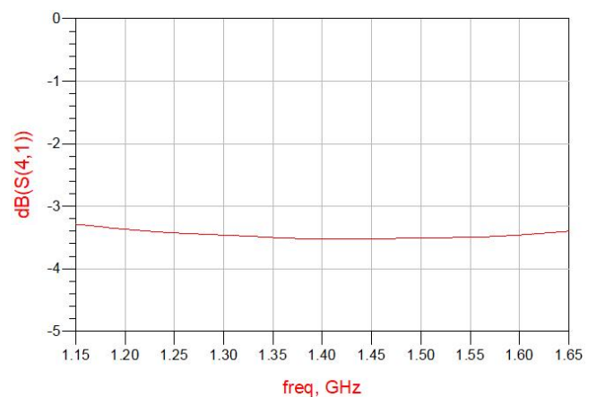
Figure 4. MHC14S03 Transmission
