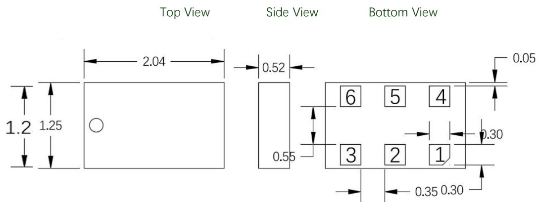
Figure 2. MHC14S03 Outline Drawing
