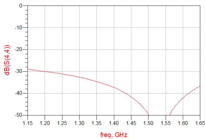
Figure 7. MHC14S03 Return Loss (S44)
