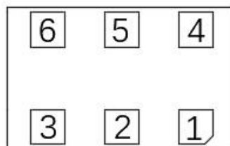
Figure 1. MHC14S03 (Bottom View)
