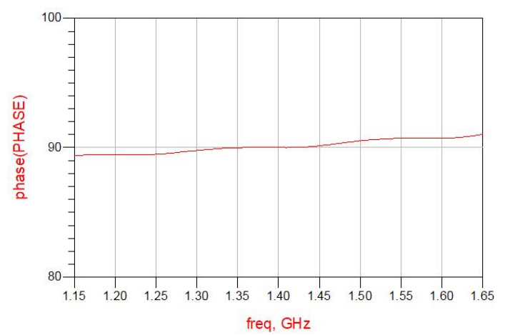
Figure 10. MHC14S03 Phase
