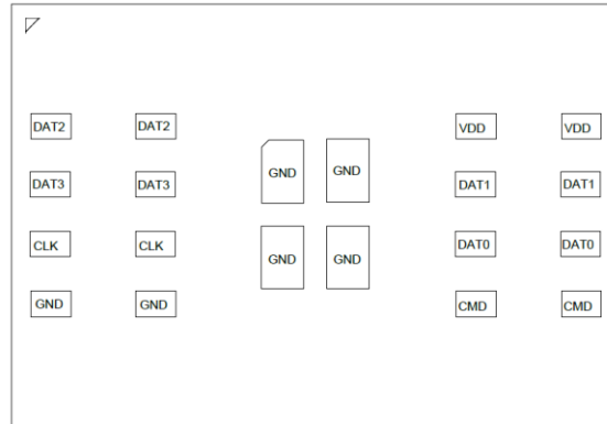
Top view through package
