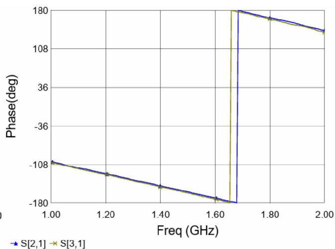
Figure 8. MPD1020W2 Phase
