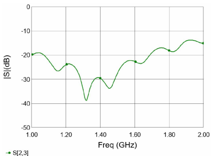
Figure 7. MPD1020W2 Isolation
