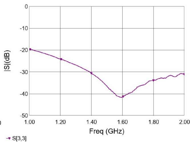
Figure 6. MPD1020W2 Return Loss (S33)
