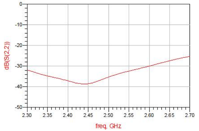
Figure 6. MHC25X02 Return Loss (S22)
