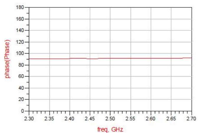
Figure 10. MHC25X02 Phase
