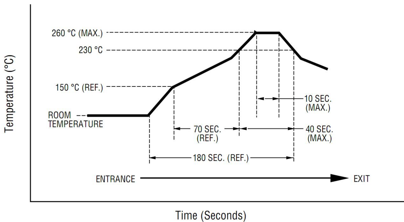
Figure 14. MHC25X02 Thermal Reflow Profile
