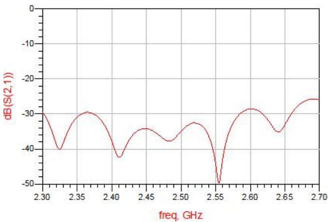
Figure 9. MHC25X02 Isolation
