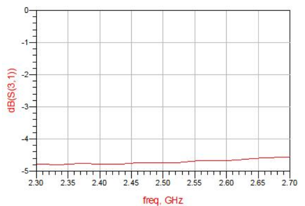
Figure 4. MHC25X02 Transmission
