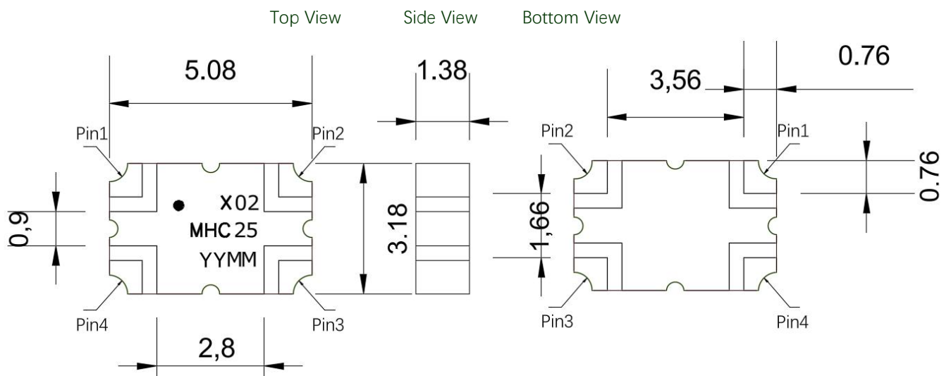
Figure 2. MHC25X02 Outline Drawing
