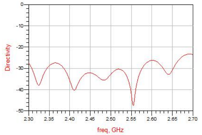
Figure 12. MHC25X02 Directivity
