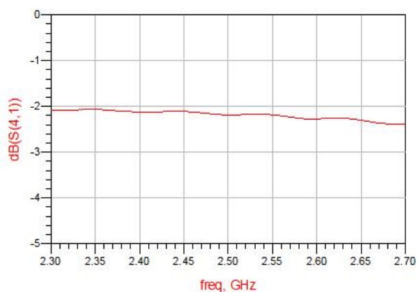
Figure 3. MHC25X02 Coupling
