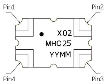
Figure 1. MHC25X02 (Top View)
