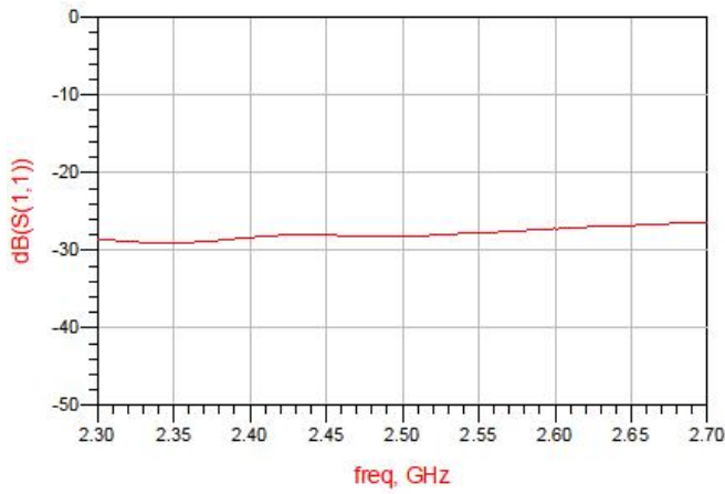
Figure 5. MHC25X02 Return Loss (S11)
