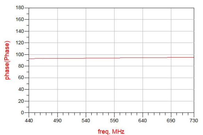
Figure 10. MHC0600L03 Phase
