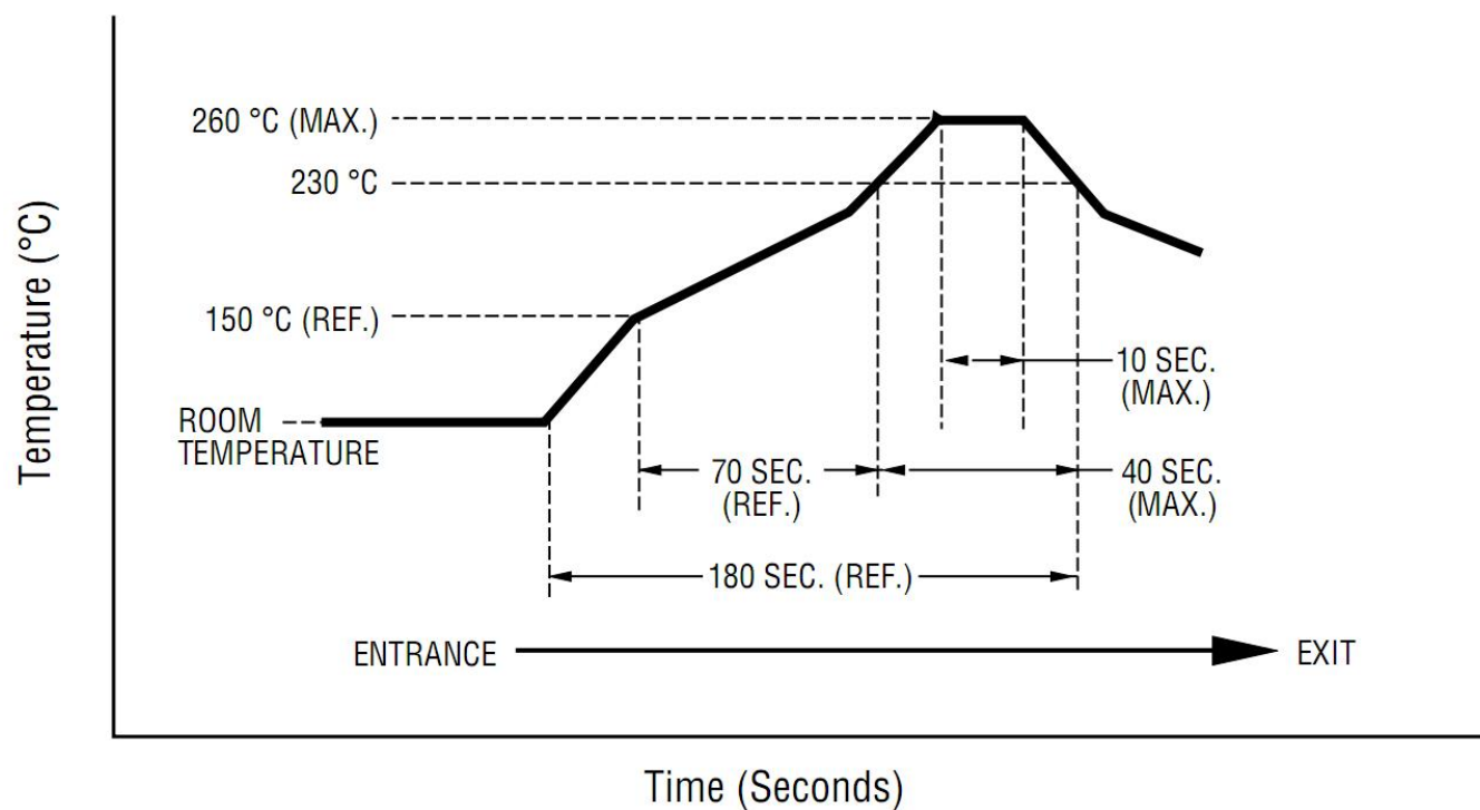
Figure 13. MHC0600L03 Thermal Reflow Profile
