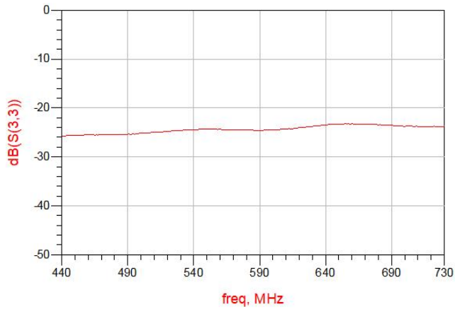
Figure 7. MHC0600L03 Return Loss (S33)
