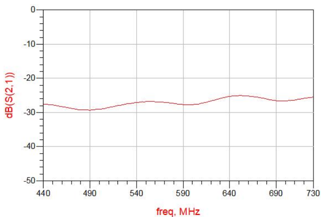
Figure 9. MHC0600L03 Isolation
