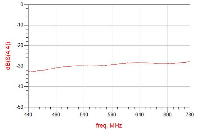
Figure 8. MHC0600L03 Return Loss (S44)
