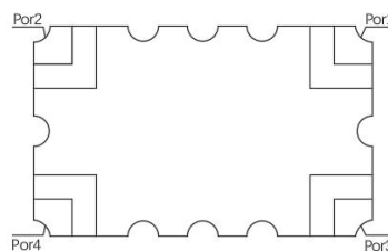
Figure 1. MHC0600L03 (Bottom View)
