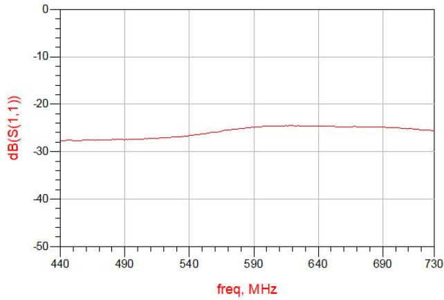
Figure 5. MHC0600L03 Return Loss (S11)
