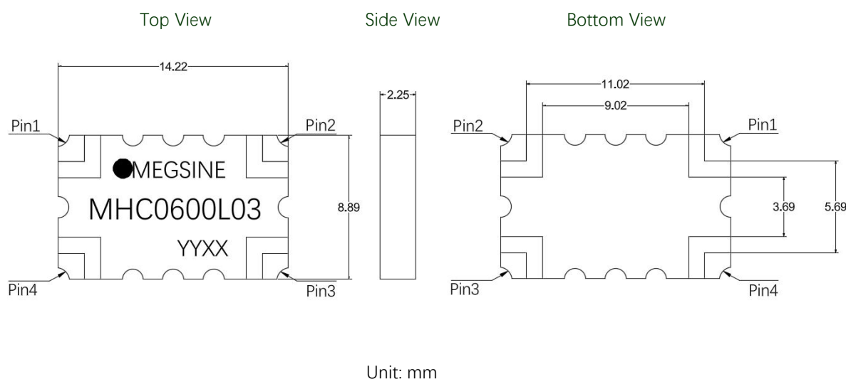
Figure 2. MHC0600L03 Outline Drawing
