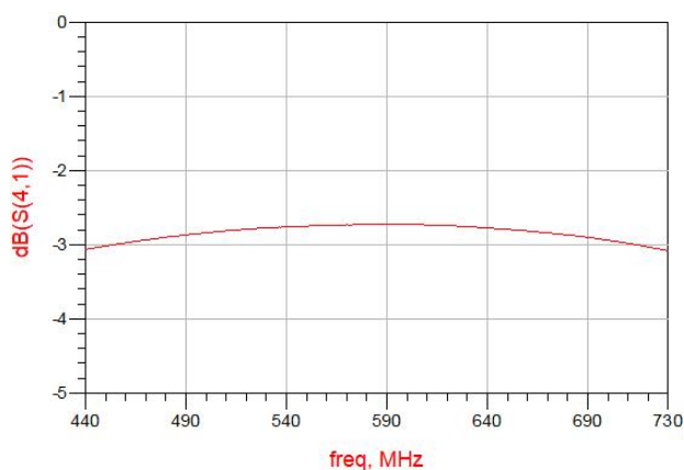
Figure 3. MHC0600L03 Coupling
