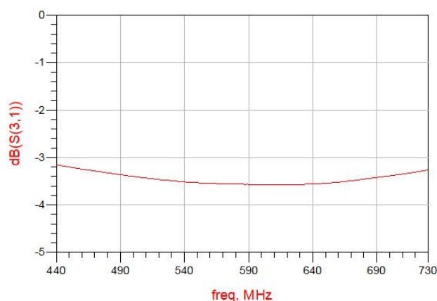
Figure 4. MHC0600L03 Transmission
