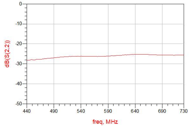
Figure 6. MHC0600L03 Return Loss (S22)
