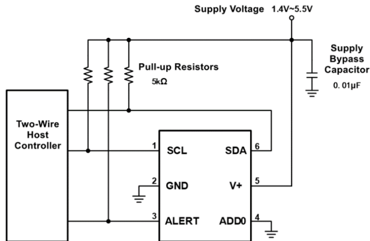
Figure 9. Typical Connections of the TMP112
