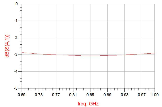
Figure 4. MHC0900L03 Transmission
