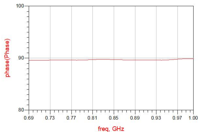
Figure 10. MHC0900L03 Phase
