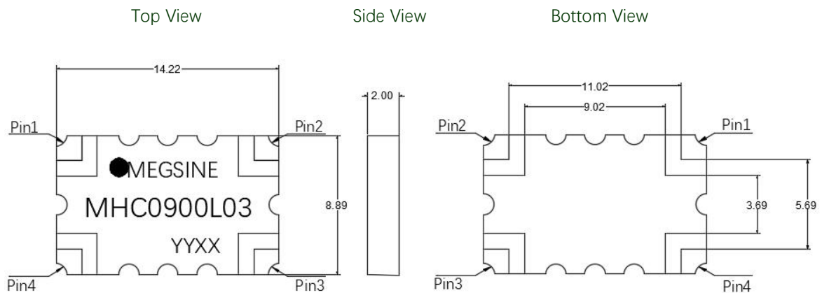
Figure 2. MHC0900L03 Outline Drawing
