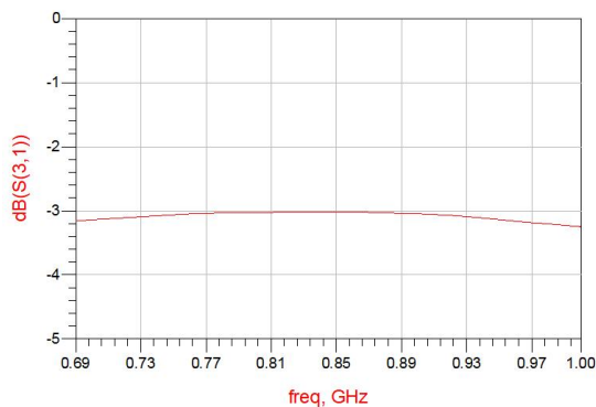
Figure 3. MHC0900L03 Coupling
