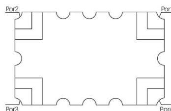
Figure 1. MHC0900L03 (Bottom View)
