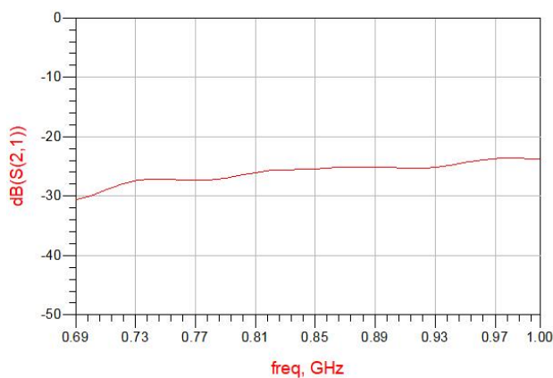
Figure 9. MHC0900L03 Isolation
