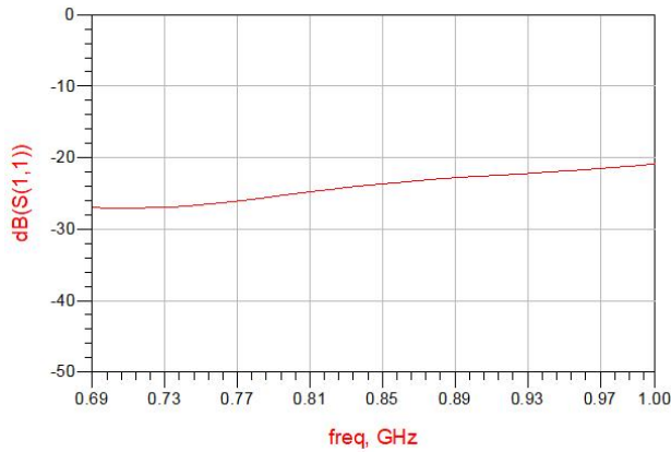
Figure 5. MHC0900L03 Return Loss (S11)
