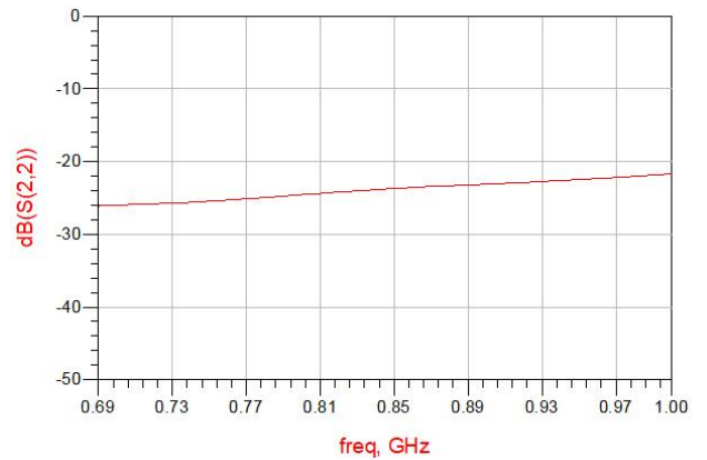
Figure 6. MHC0900L03 Return Loss (S22)
